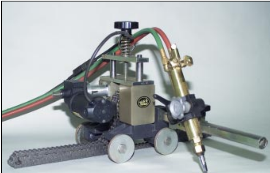
Motorized Pipe-Bug 110V. Part # BUG-05-0520-M00 Weight: 42lbs (19kg) Shipping Weight: 47 lbs. (22kg)
